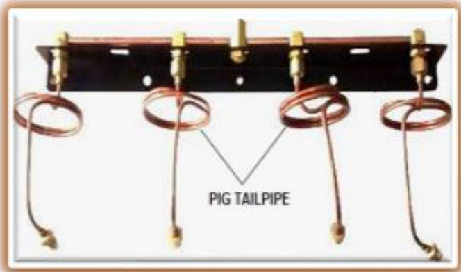
OXYGEN MANIFOLD
